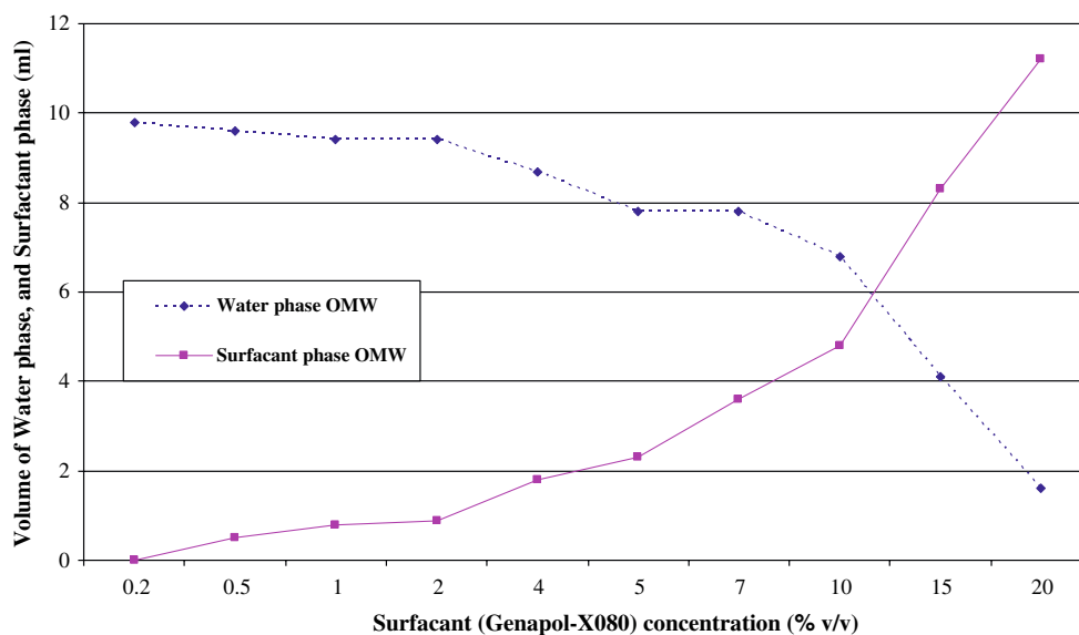
Fig. 2 The relationship between the measured volume of water and surfactant phases after centrifugal separation and surfactant concentration (% v/v-Genapol X-080)
