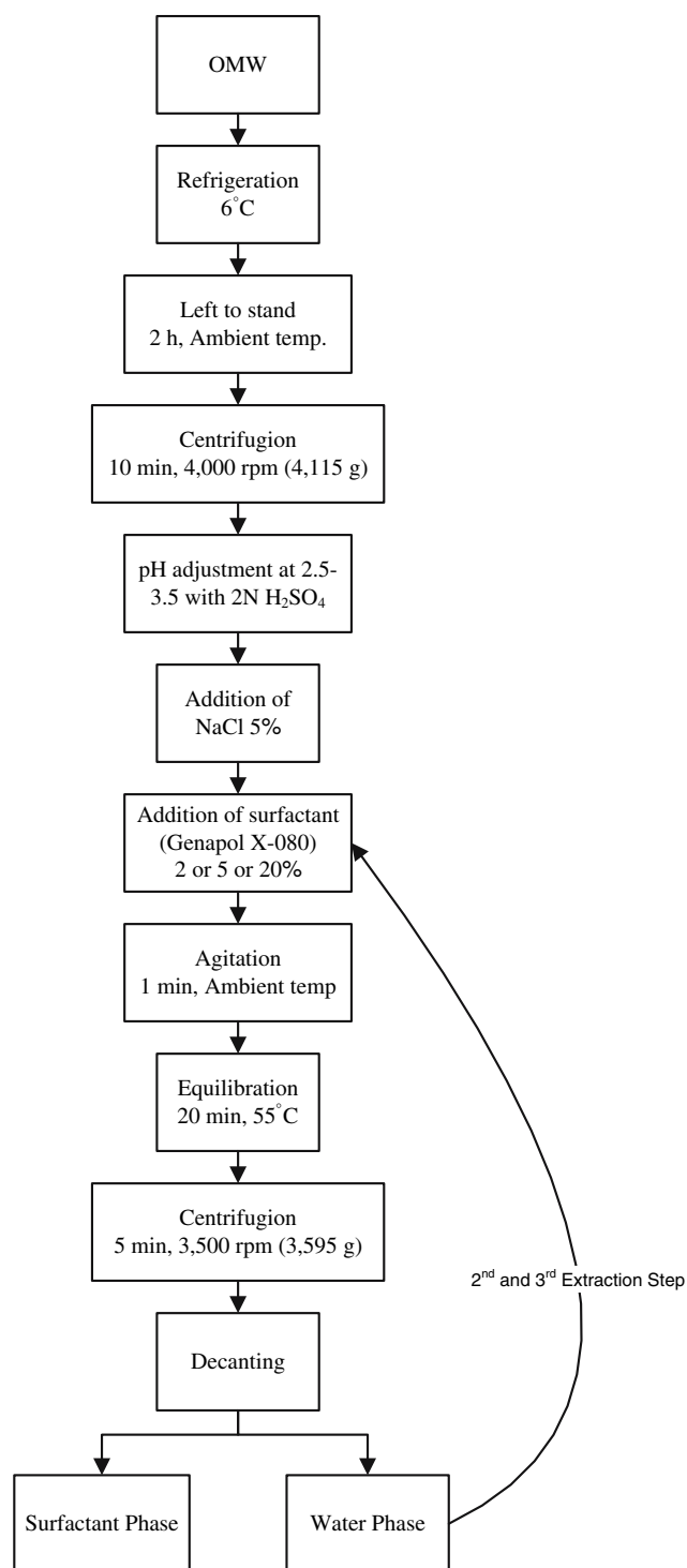
Fig. 1 Schematic representation of the CPE procedure
